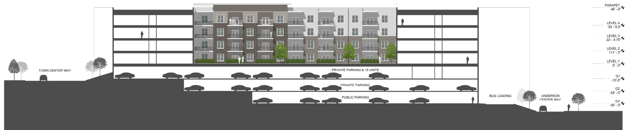
East Courtyard Elevation and Building Section
